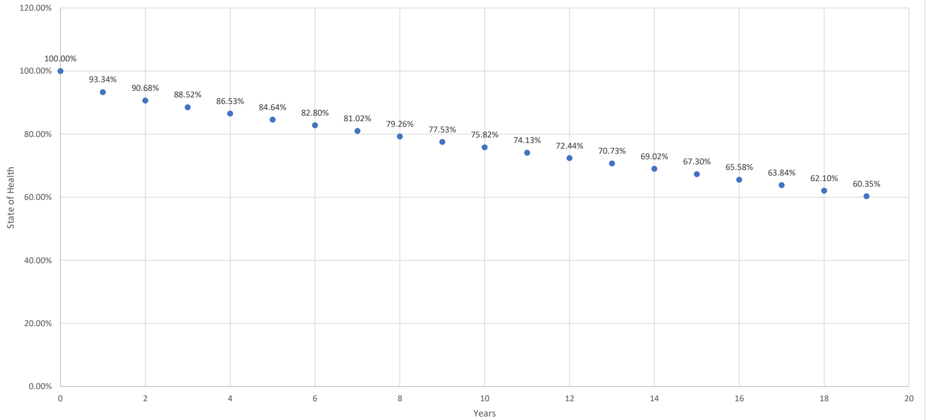
SOH LUNA2000-200KWH-2H1 0.5C, 1 cycle/day
